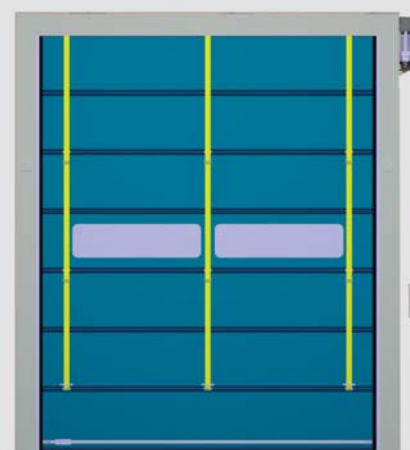
Door's rear view showing the vertical belts connected to the ribs.
