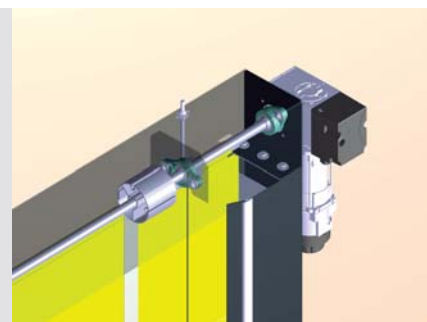
Motor attached to door's frame.
